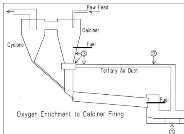
Figure 2: oxygen injection points
